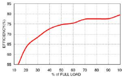
FKC05-48S05 Efficiency vs. Output Load
